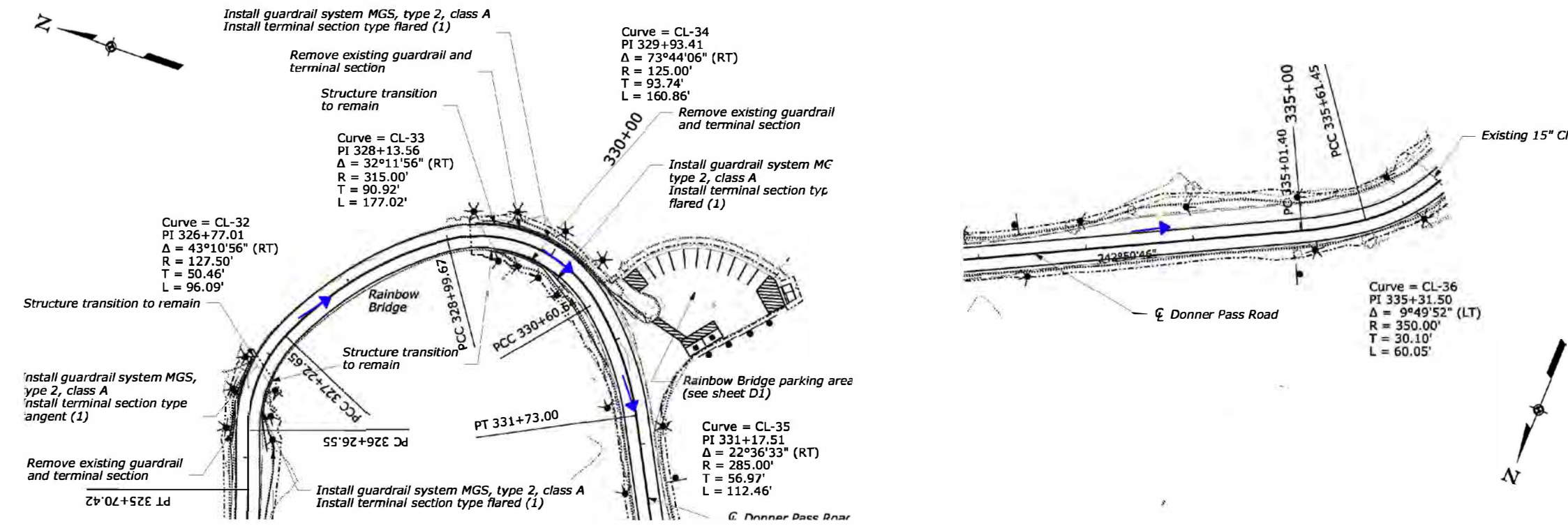
From 326+00 to 336+00
