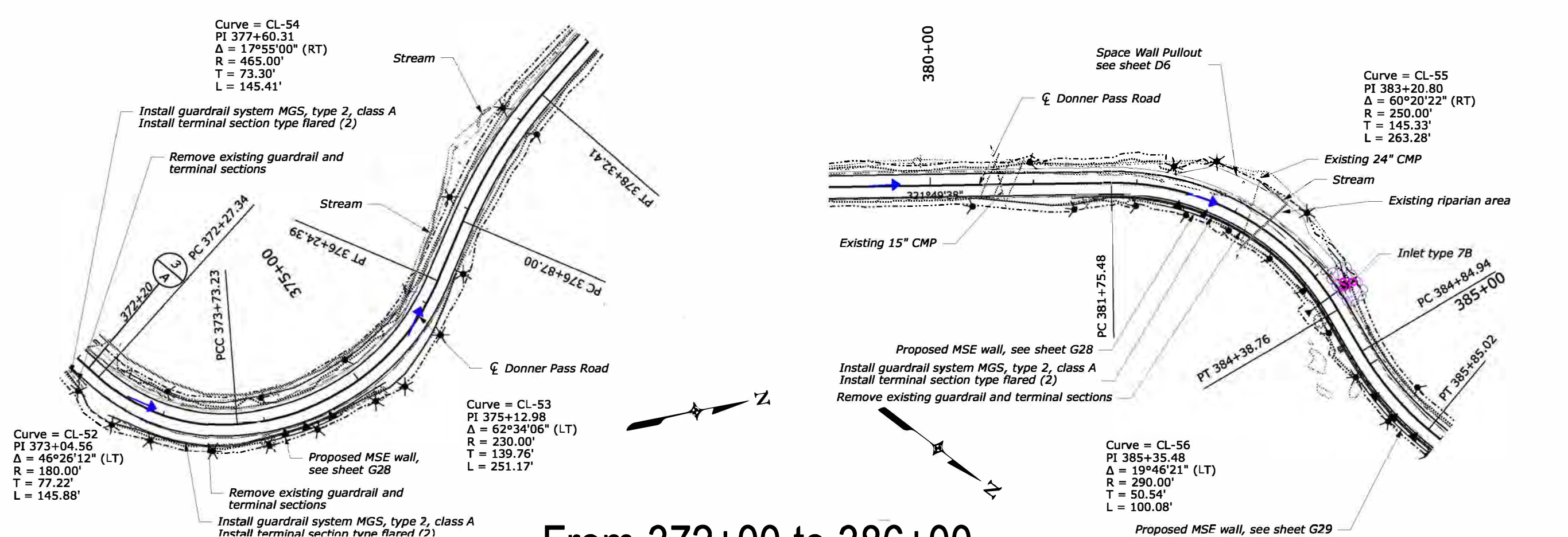
From 372+00 to 386+00
