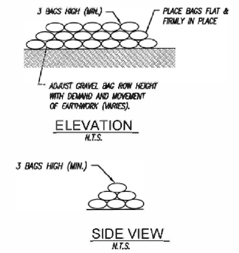
Gravel Bag Berm (SE-6)
