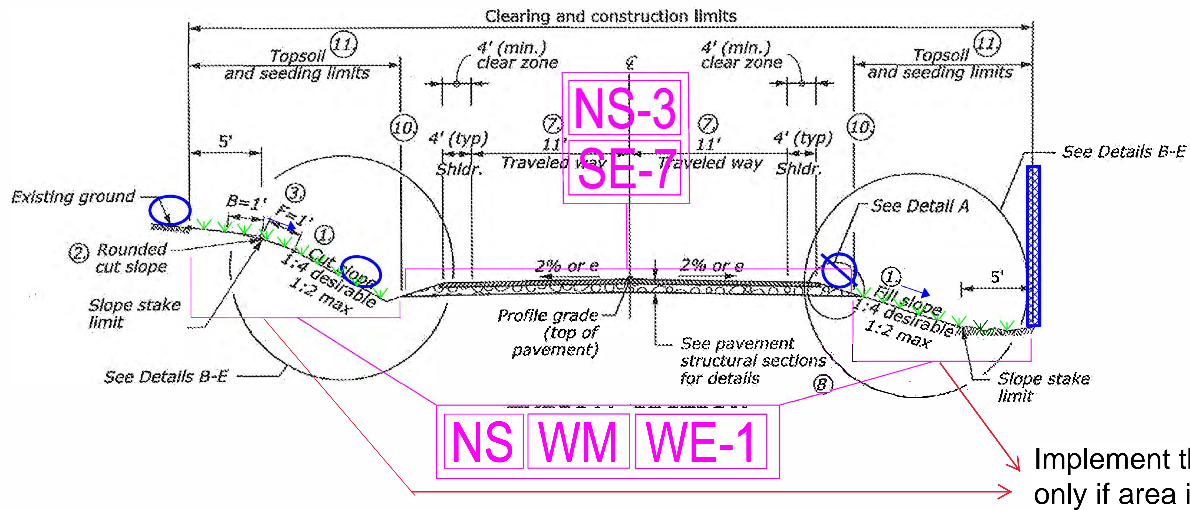
Typical BMP Implementation throughout the site
