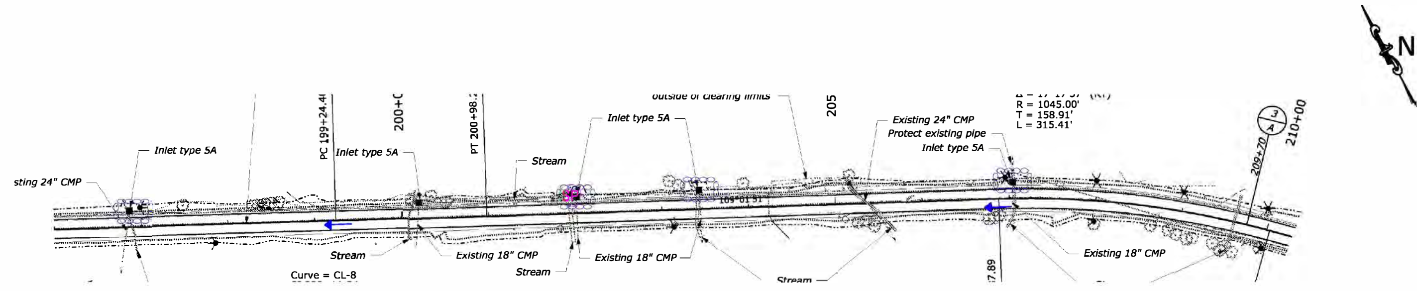
From 196+00 to 210+00
