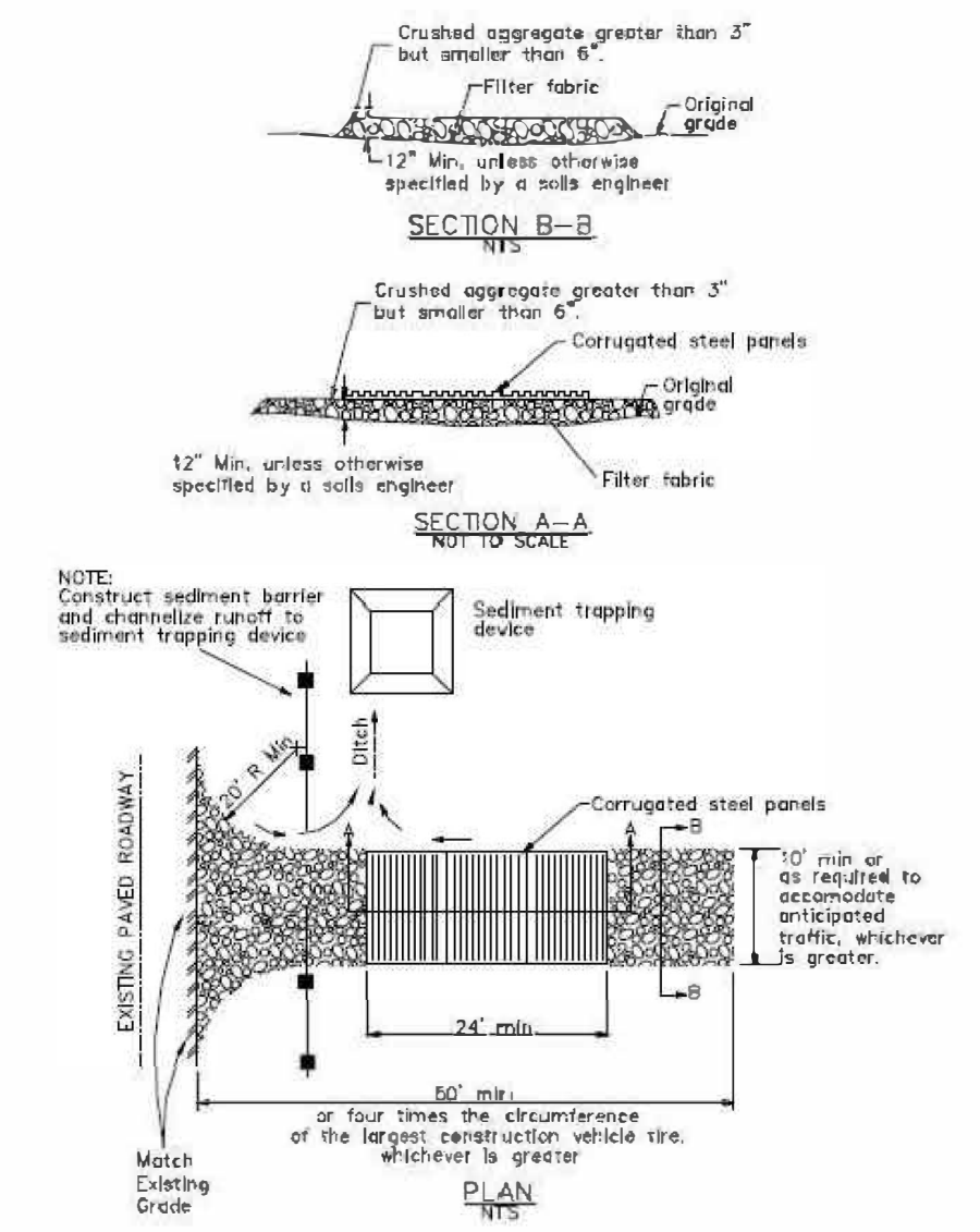
Stabilized Construction Entrance/Exit (TC-1)
