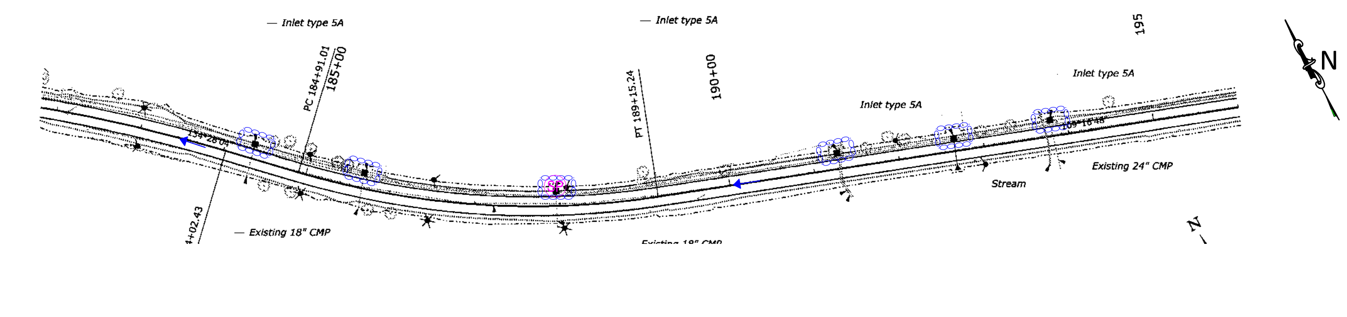
From 182+00 to 196+00
