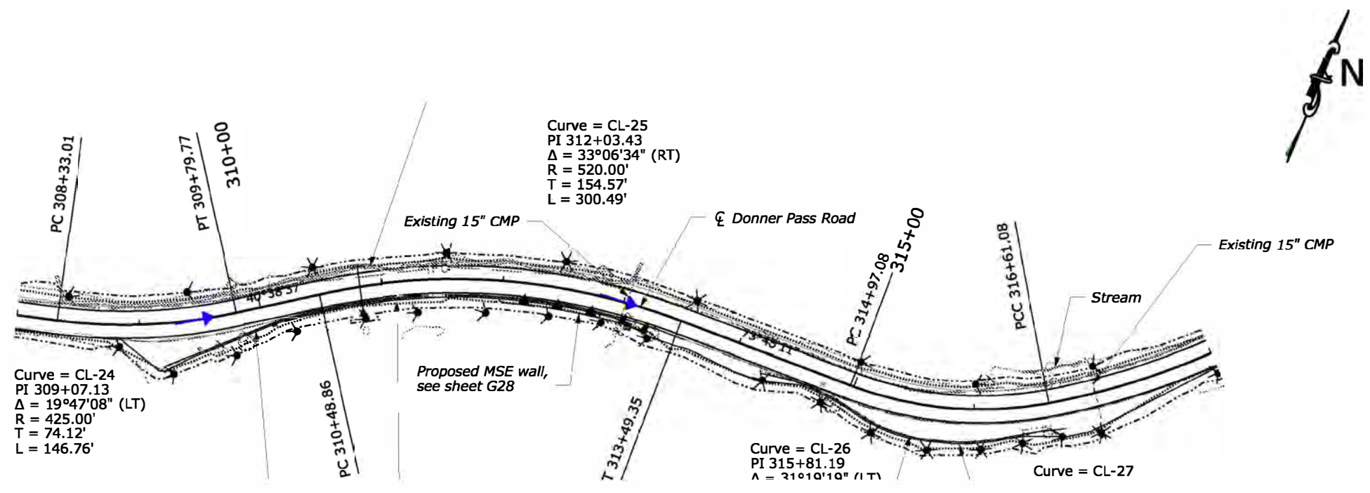
From 308+00 to 318+00
