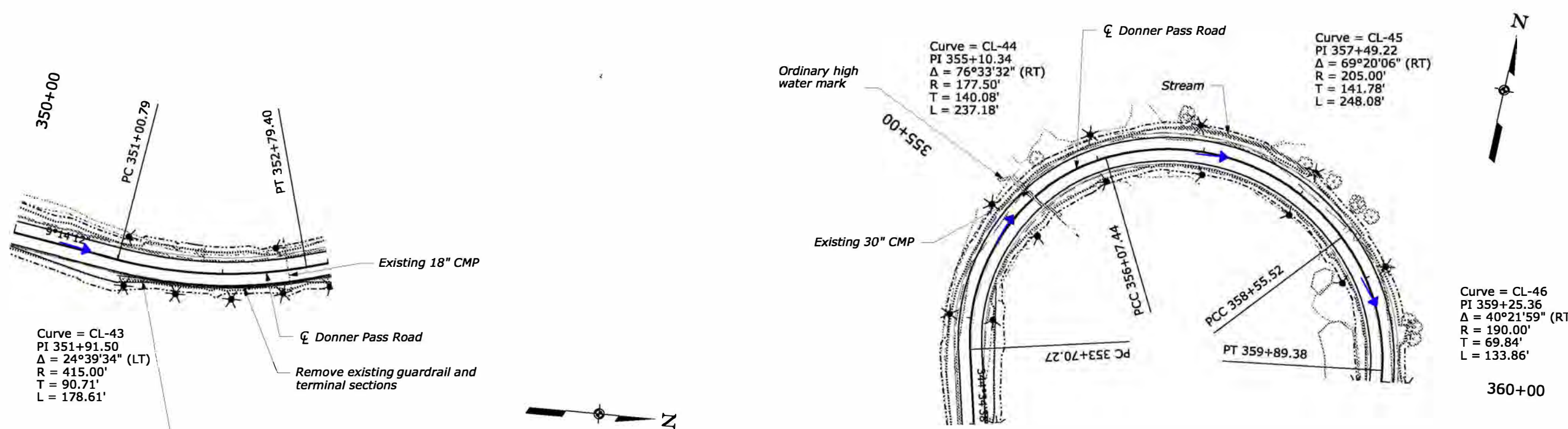
From 350+00 to 360+00
