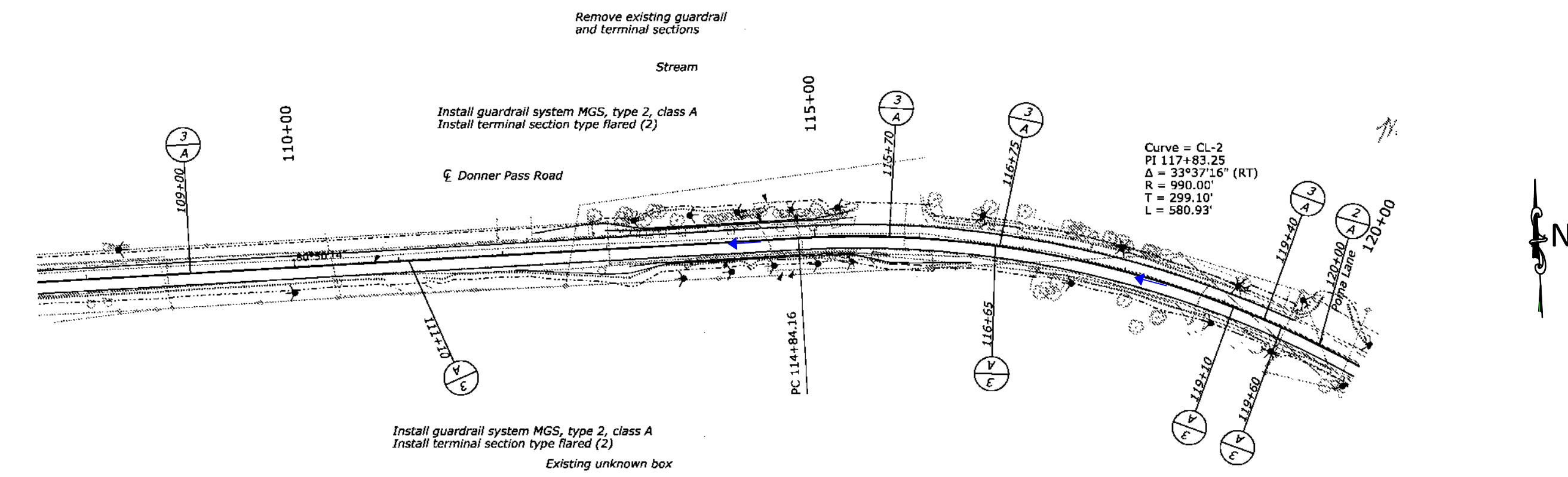
From 108+00 to 120+00
