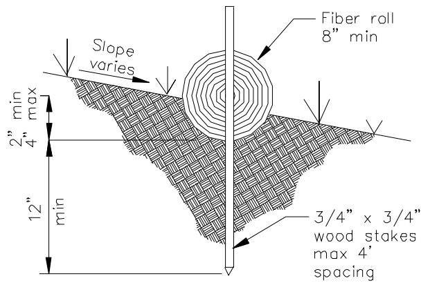
ENTRENCHMENT DETAIL
