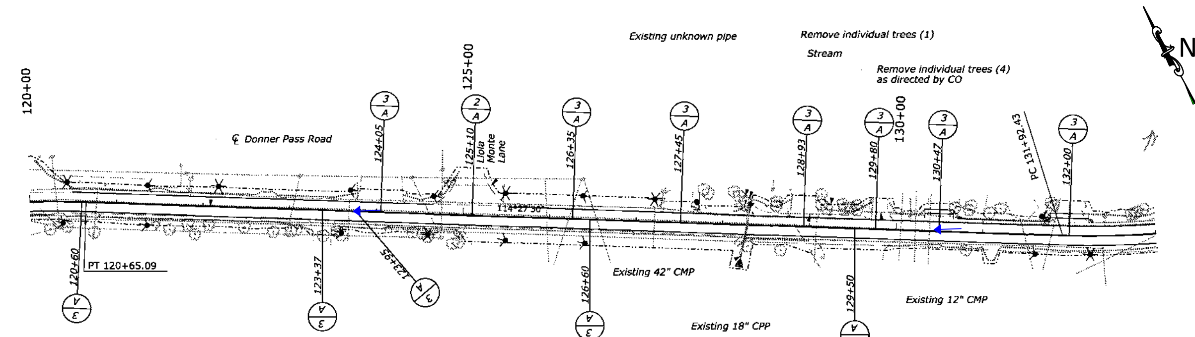
From 120+00 to 133+00
