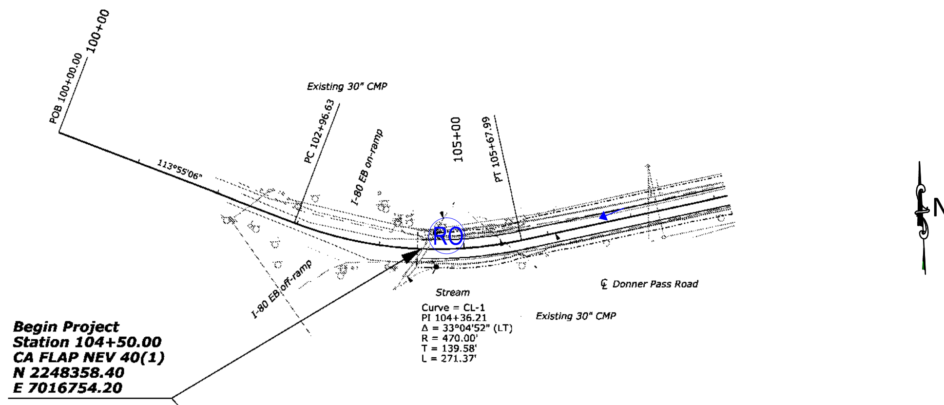
From 104+50 to 108+00
