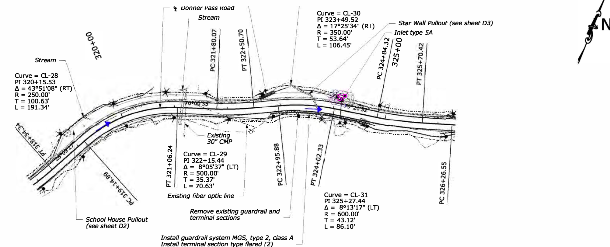
From 318+00 to 326+00
