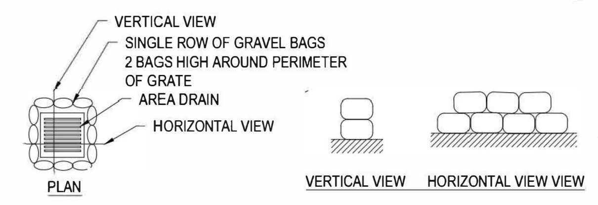
Inlet Protection (SE-10)
