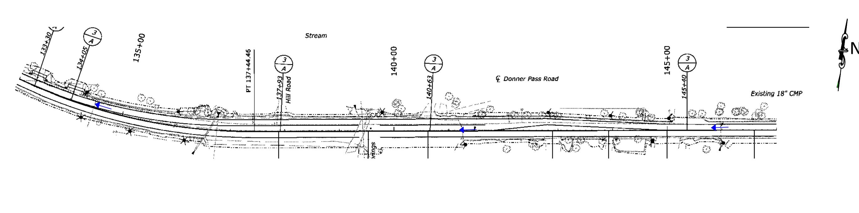
From 133+00 to 147+00
