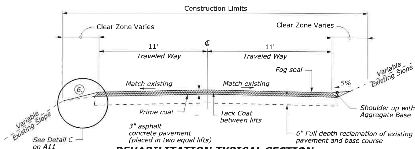
REHABILITATION TYPICAL SECTION REDS MEADOW ROAD 496+69.57 to 713+10.00 725+30.00 to 805+57.87
