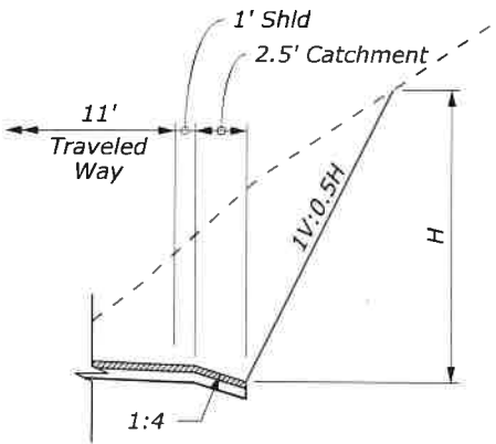
ROCK EXCAVATION DETAIL 2 ⑤ H \leq 10'
