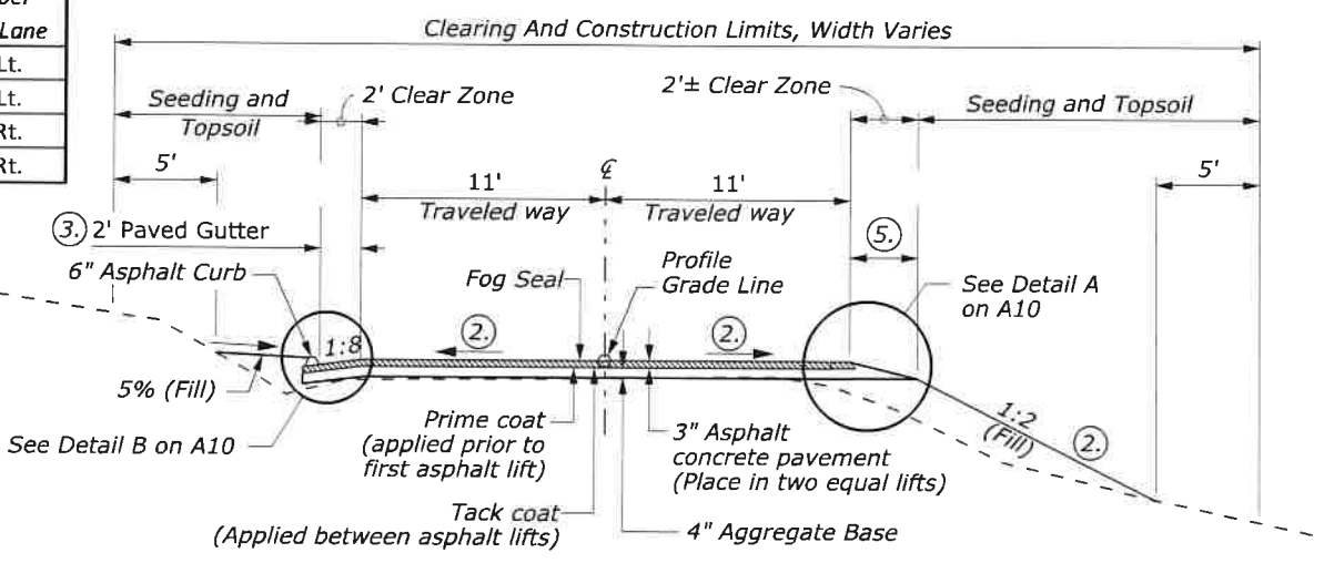
TYPICAL SECTION REDS MEADOW ROAD 713+10 TO 725+30.00
