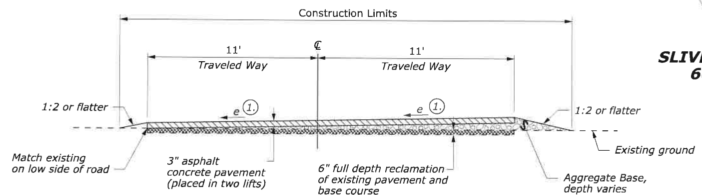
SUPERELEVATION CORRECTION TYPICAL SECTION REDS MEADOW ROAD
