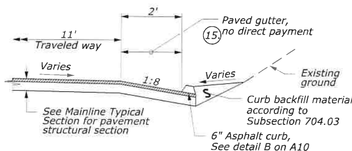
PAVED GUTTER DETAIL 648+60 to 649+05, Lt 714+60 to 722+72, Lt 786+98 to 797+05, Lt
