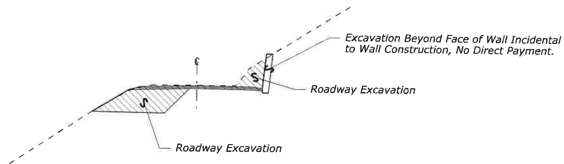
ROADWAY EXCAVATION
