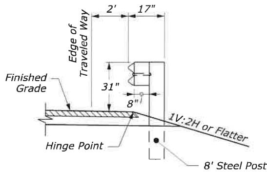
GUARDRAIL DETAIL 1 USE ON 1:2 OR FLATTER SLOPES
