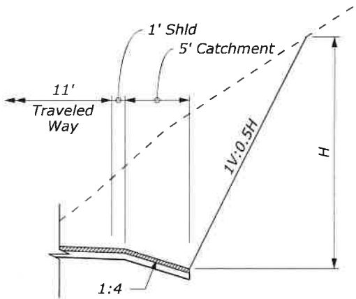
ROCK EXCAVATION DETAIL 1 ⑤ 10' < H \leq 20'
