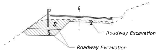
ROADWAY EXCAVATION
