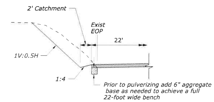
ROCK EXCAVATION DETAIL 580+00 TO 584+50 694+00 TO 694+20.00
