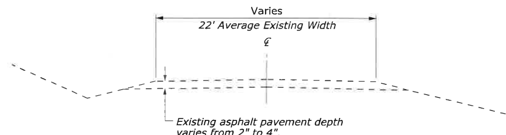
EXISTING TYPICAL SECTION 496+69.57 to 805+57.87
