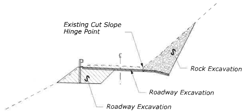
ROCK EXCAVATION
