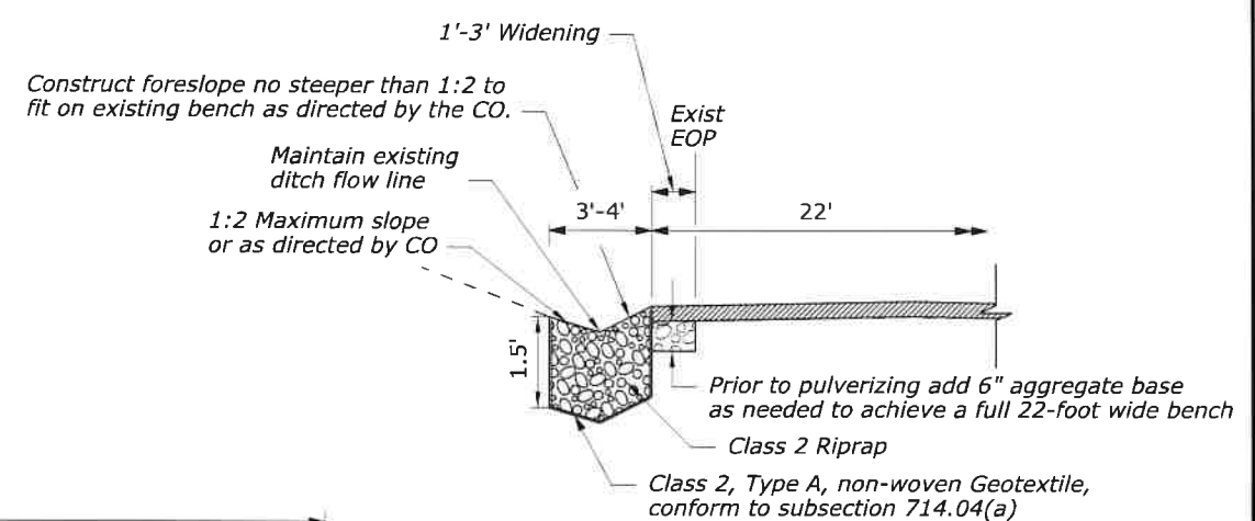
SLIVER WIDENING DETAIL 604+00 TO 608+50
