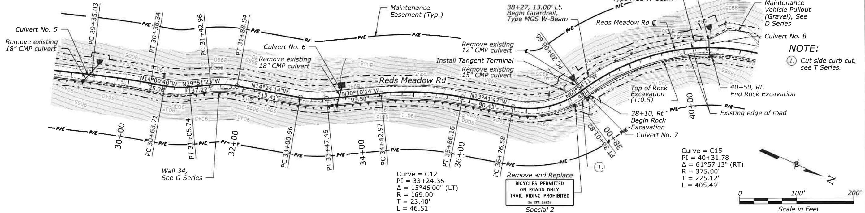
Superelevation Diagram
