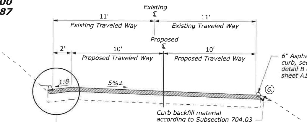
HIGH SIDE CURB DETAIL 786+98 to 797+05, Lt 790+05 to 796+05, Rt
