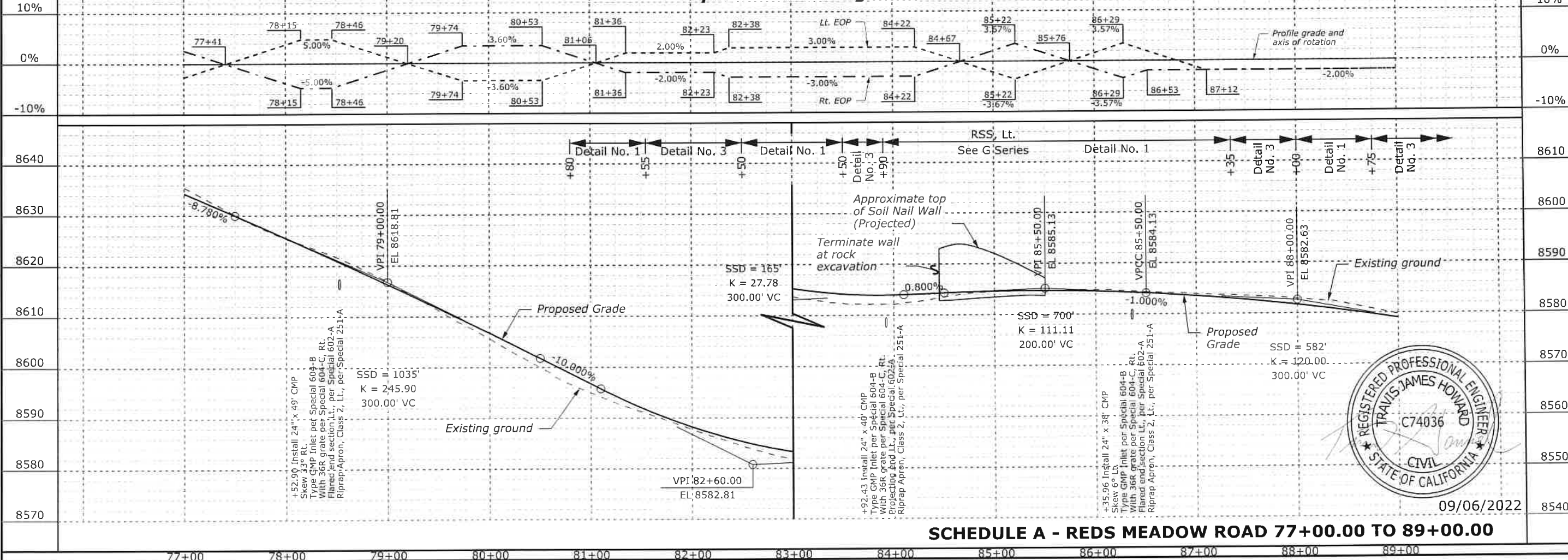
Superelevation Diagram
