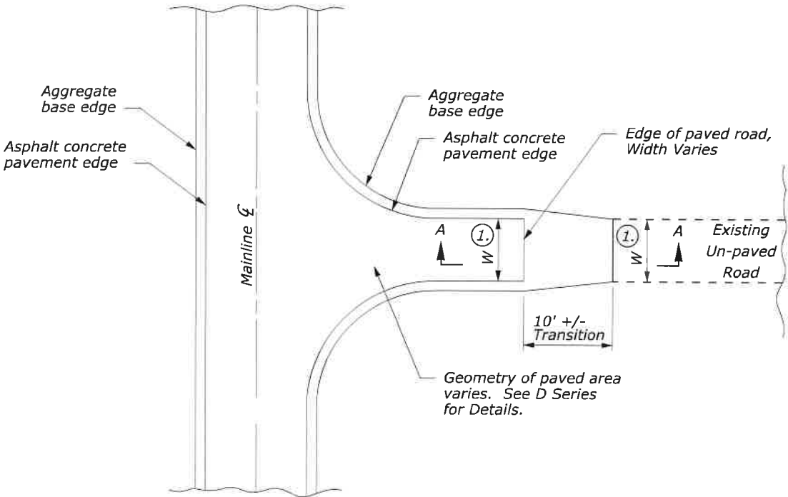
TYPICAL PLAN
