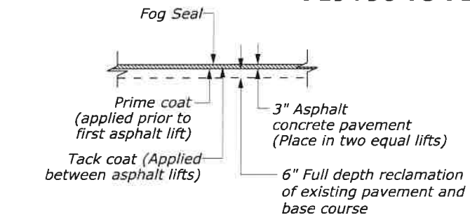
TYPICAL SECTION BUS STOPS AND DRIVEWAYS
